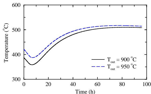
Figure 2. Maximum reactor vessel temperatures during a depressurized conduction cooldown accident with the prismatic design.
