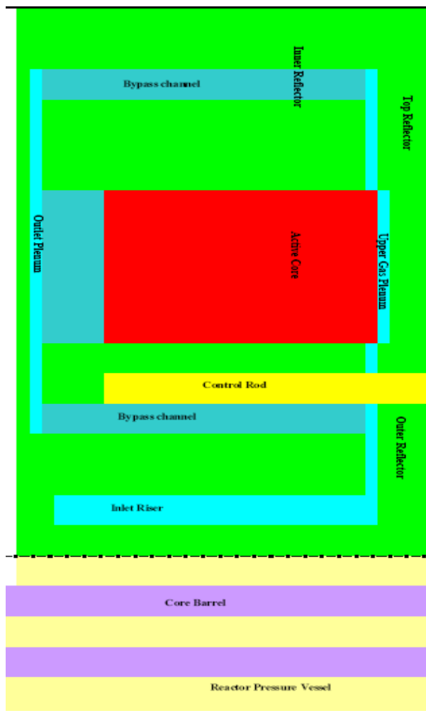
Figure 5: THERMIX model of 600 MW Pebble-bed VHTR
