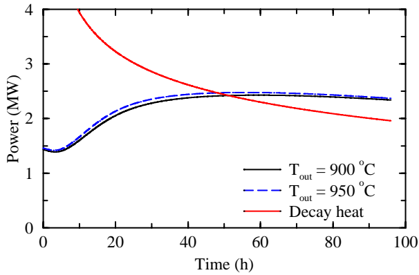
Figure 9. A comparison of RELAP5-3D calculated RCCS heat removal and core decay power during a depressurized conduction cooldown accident with the pebble-bed design.
