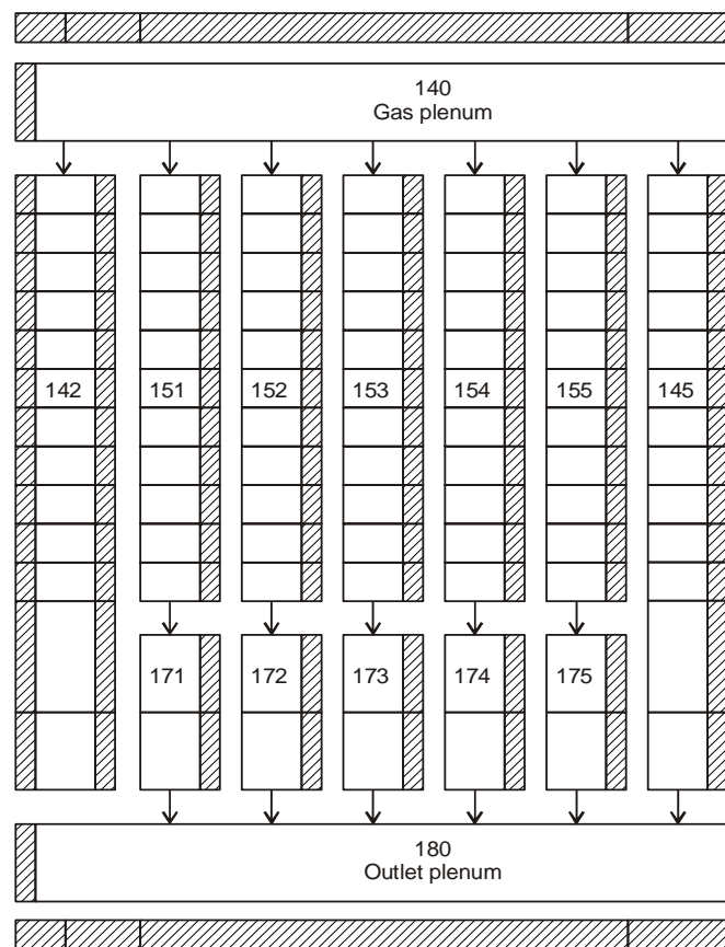
Figure 6. RELAP5-3D model of the pebble-bed design.
